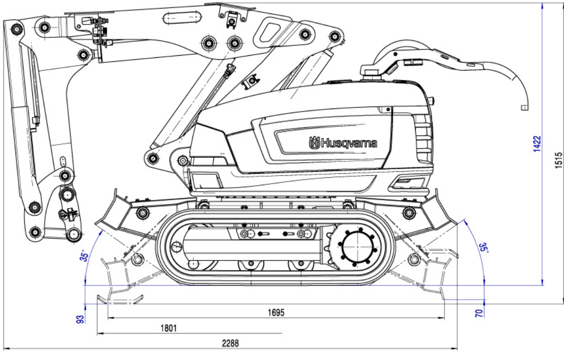
The DXR 250, measurements.
