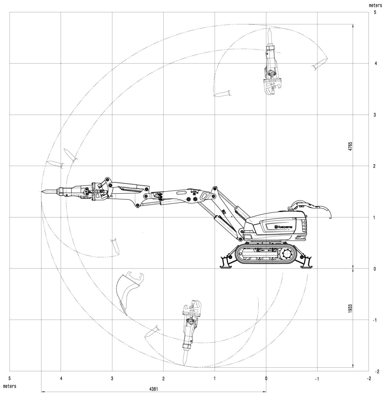
Range, the DXR 250: approx. 4,5 meters.
