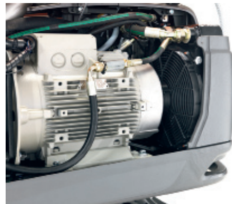
Cool. The electrical fan gives efficient cooling, and results in a machine of high efficiency.
