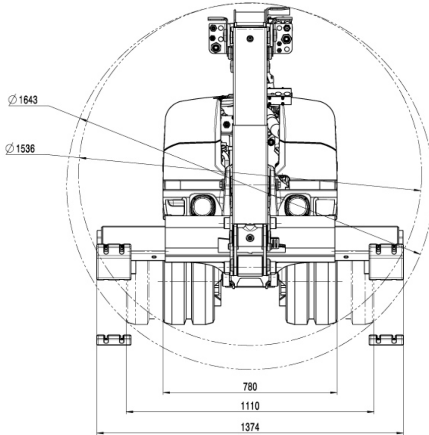
The DXR 250, dimension of body, width: 780 mm.
